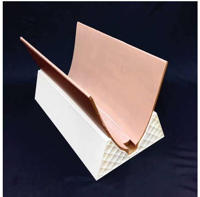
Figure 12. ULTEM 1010 layup tool nested into ASA cradle.
