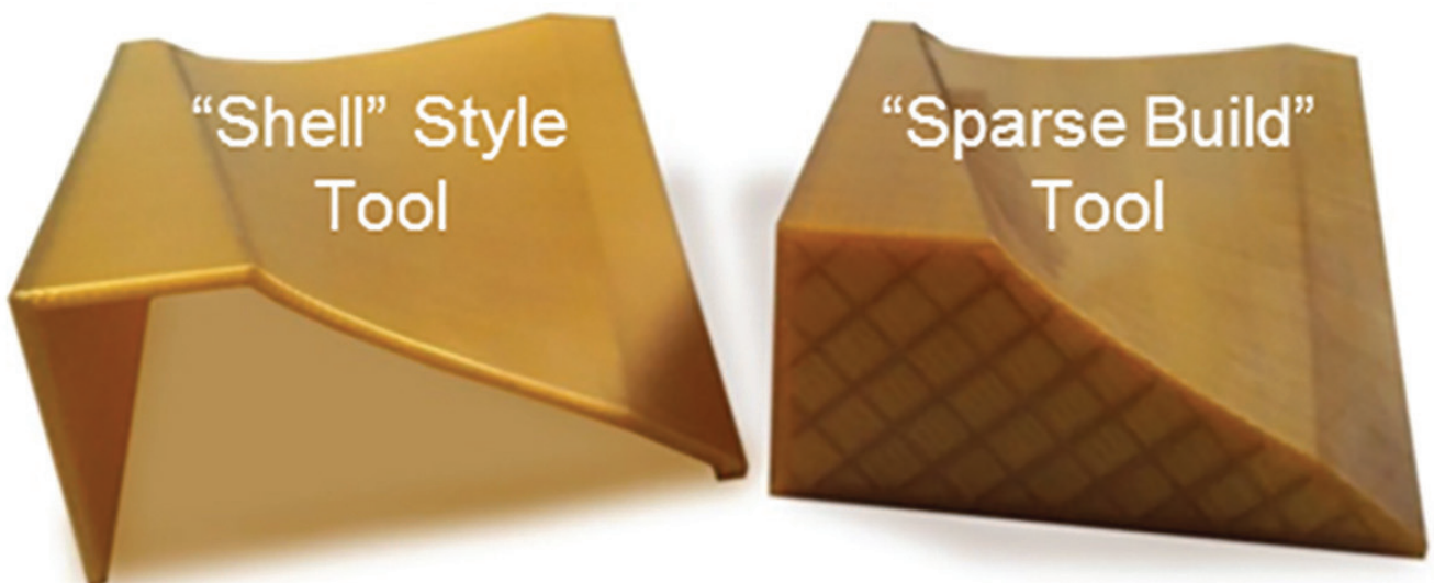
Figure 1. Shell and sparse style tools.
