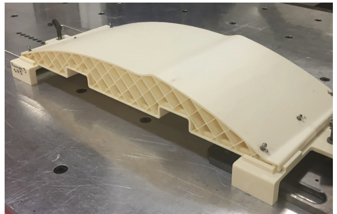
Figure 7 (Middle Right). FDM machining fixture secured to the CNC platen.
