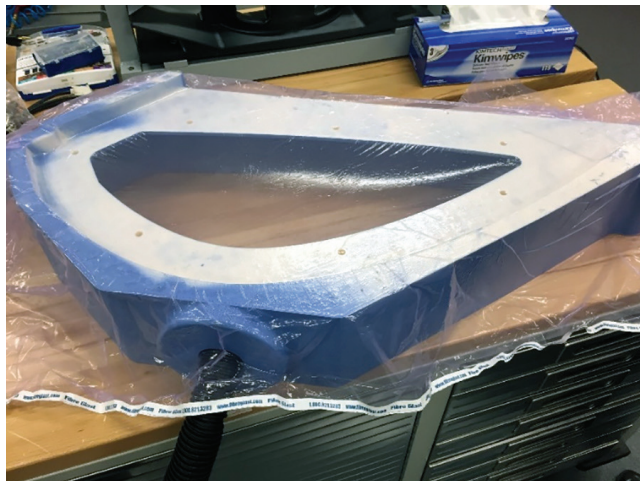
Figure 11. Test setup to evaluate the effectiveness of using spray paint to effectively seal the edges of the vacuum fixture.
